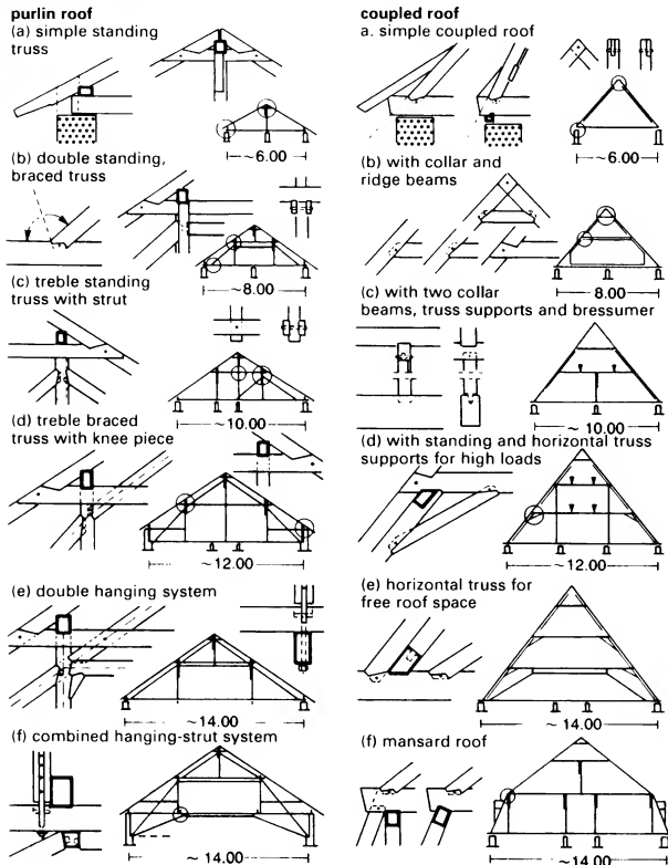
② Designs of purlin and coupled roofs
